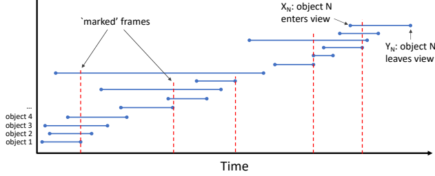
Figure 4: Visualizing objects entering and leaving an AV’s view. Dashed lines represent frames chosen by the min-frame algorithm.
