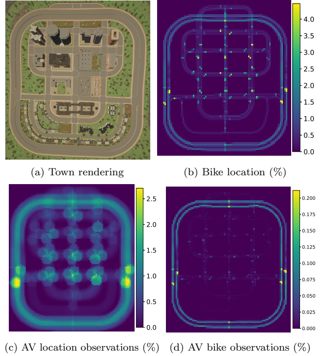
Figure 5: Carla simulation with one AV and 17 bikes over 48 hours. 5b shows the percentage of time a bike is within each 5×5m cell, 5c shows the percentage of time each location is observed by an AV, and 5d shows how often a bike is observed by an AV.
