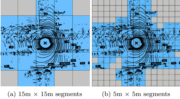
Figure 7: Aerial view of a LIDAR point cloud, from [40]. "X" marks the location of the LIDAR sensor, and rectangles mark the location of observed vehicles. Smaller segments offer higher specificity of which areas are observed (blue), providing a more accurate sampling distribution estimate for each location.
